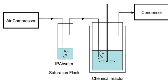
Figure 7. IPA/H 2 O-saturated air sparge.
