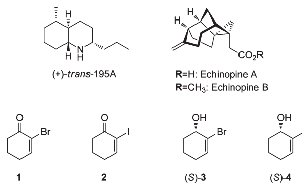
Figure 1. Recent natural product synthesis targets, (+)- trans -195A and echinopines A and B, which require (S)- 3 or (S)- 4 as intermediates derived from ketones 1 or 2 , respectively.
