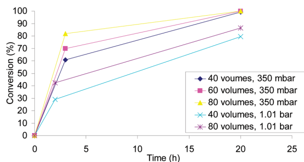
Figure 6. Effect of reduced pressure at a range of substrate loadings on the reduction of ketone 1 to afford alcohol (S)- 3 .
